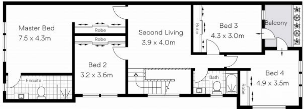
First Floor
