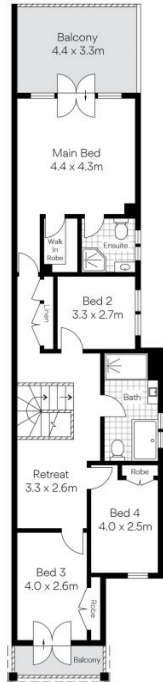
First Floor
