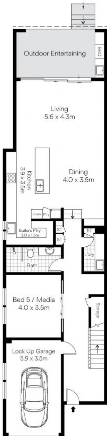
Ground Floor
